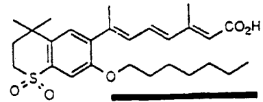
Ro 46-8515
